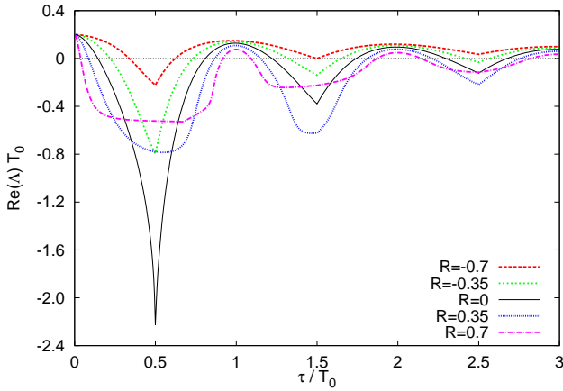
Fig. 1. (Color online) Largest real part of the complex eigenvalues \Lambda as a function of \tau for different values of R . The red, green, black, blue, and magenta curves correspond to R = -0.7, -0.35, 0, 0.35, 0.7 , respectively. The parameters of the unstable focus are chosen as \lambda = 0.1 and \omega = \pi which yields an intrinsic period T_0 = 2\pi/\omega = 2 . The feedback gain K is fixed at KT_0 = 0.6 .
