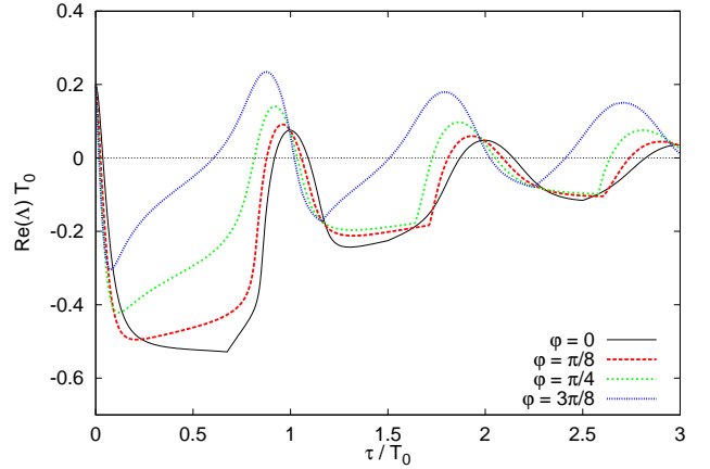
Fig. 5. (Color online) Largest real part of the eigenvalues \Lambda as a function of \tau for different phases \varphi . The black, red, green, and blue curves correspond to \varphi = 0, \pi/8, \pi/4 , and 3\pi/8 , respectively. The other control parameters are fixed as R = 0.7 and KT_0 = 0.6 . The parameters of the system are as in Fig. 1.
