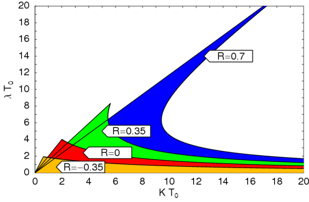
Fig. 4. (Color online) Domain of control in the (K, \lambda) plane for different memory parameters R . The yellow, red, green, and blue areas correspond to R = -0.35, 0 (TDAS), 0.35 , and 0.7 , respectively. The time delay is fixed at \tau = T_0/2 .
