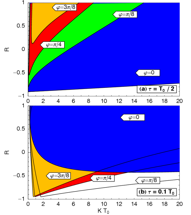
Fig. 8. (Color online) Domain of control in the (K, R) plane for different values of the feedback phase \varphi . The blue, green, red, and yellow areas correspond to \varphi = 0, \pi/8, \pi/4 , and 3\pi/8 , respectively. Panel (a) displays the domain of control for optimal \tau = T_0/2 ; panel (b) for \tau = 0.1T_0 . The parameters of the system are as in Fig. 1.
