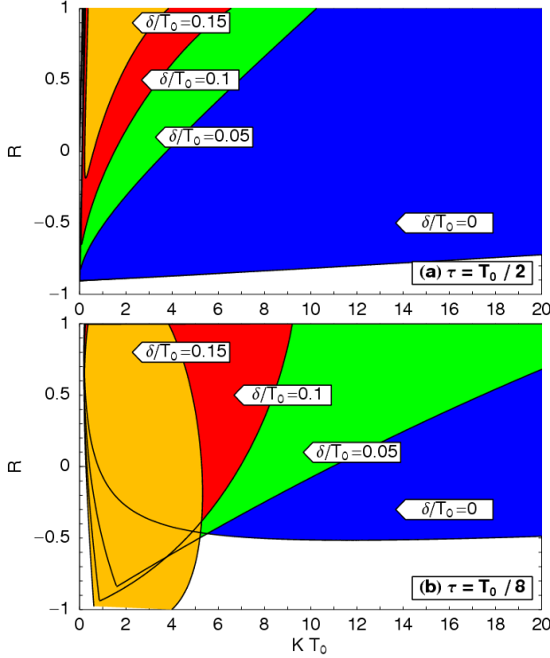
Fig. 11. (Color online) Domain of control in the (K, R) plane for different values of the latency time \delta . The blue, green, red, and yellow areas refer to values of \delta = 0, 0.05T_0, 0.1T_0 , and 0.15T_0 , respectively. Panel (a) corresponds to an optimal time delay \tau = T_0/2 , panel (b) to \tau = T_0/8 . The parameters of the system are as in Fig. 1.
