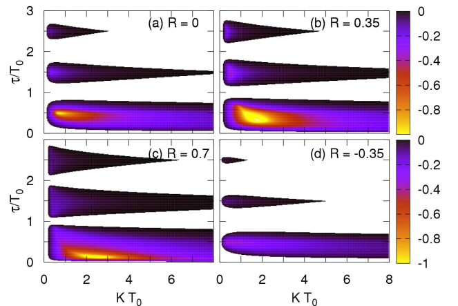
Fig. 2. (Color online) Domain of control in the (K, \tau) plane for different values of R : 0, 0.35, 0.7, -0.35 in panels (a), (b), (c), and (d), respectively. The greyscale (color online) shows only negative values of the largest real part of the complex eigenvalues \Lambda according to Eq. (6). The parameters of the system are as in Fig. 1.
