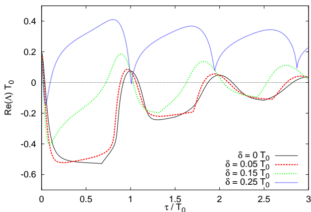
Fig. 9. (Color online) Largest real part of the eigenvalues \Lambda as a function of \tau for different latency times \delta . The black, red, green, and blue curves correspond to \delta = 0, 0.05T_0, 0.15T_0, and 0.25T_0 , respectively. The other control parameters are fixed as R = 0.7 and KT_0 = 0.6 . The parameters of the system are as in Fig. 1.
