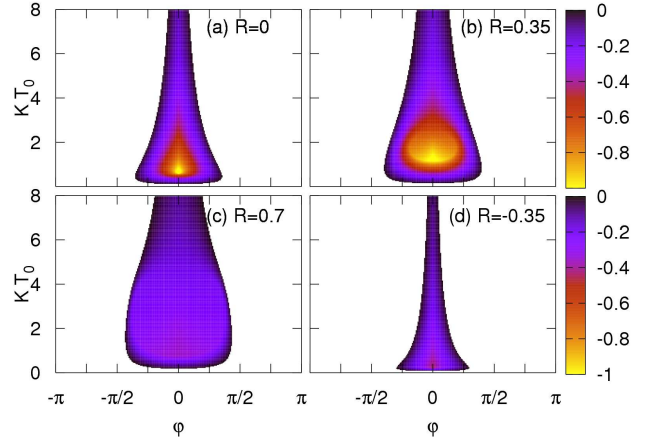
Fig. 6. (Color online) Domain of control in the (\varphi, K) plane for optimal time delay \tau = T_0/2 . Panels (a), (b), (c), and (d) correspond to a memory parameter R of 0, 0.35, 0.7 , and -0.35 , respectively. The color code shows the largest real part of the complex eigenvalues \Lambda as given by Eq. (21). The parameters of the system are as in Fig. 1.
