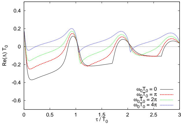
Fig. 13. (Color online) Largest real part of the eigenvalues \Lambda as a function of \tau for different mean values of the filter \omega_0 and fixed \gamma T_0 = 10 . The black, red, green, and blue curves correspond to \omega_0 T_0 = 0, \pi, 2\pi, and 4\pi, respectively. The other control parameters are fixed as R = 0.7 and KT_0 = 0.6 . The parameters of the system are as in Fig. 1.
