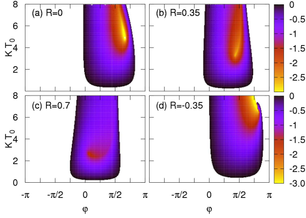
Fig. 7. (Color online) Domain of control in the (\varphi, K) plane for time delay \tau = 0.1T_0 . Panels (a), (b), (c), and (d) correspond to a memory parameter R of 0, 0.35, 0.7, and -0.35 , respectively. The color code shows the largest real part of the complex eigenvalues \Lambda as given by Eq. (21). Only negative values are depicted. The parameters of the system are as in Fig. 1.
