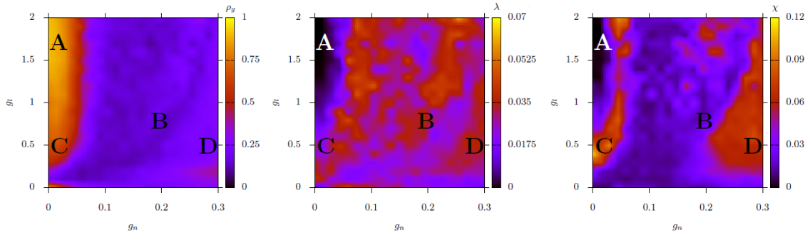
Figure 1. Parameter spaces in the (g_n, g_l) parameter space for the global order parameter (left), the metastability index (middle) and the chimer-like index (right).
