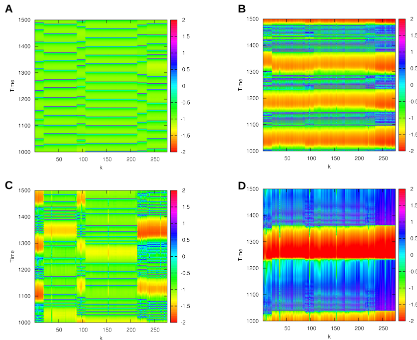
Figure 2. Space-time plots of the whole network for the 4 points marked in the parameter spaces of Fig. 1. A : \lambda and \chi very low, B : \lambda high, \chi low, C : \chi high, \lambda low, D : \chi and \lambda of same medium value. Node indices have been reordered.
