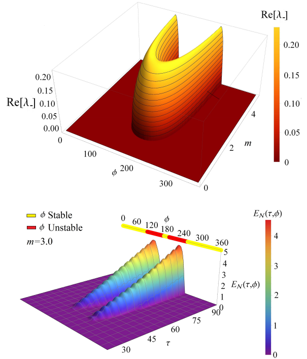
Figure 4. (Top) Map of Floquet exponent and (Bottom) Logarithmic Negativity E_N in term of phase and amplitude of perturbation.
