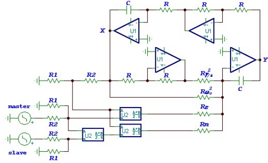
Figure 1. Circuitual implementation of Mathieu oscillator and its phase control. U_1 = LT1114CN , U_2 = MLT04G , R_{\gamma^2/4} = 438k\Omega , R_{\omega_o^2} = 39k\Omega , R_{\varepsilon} = 51k\Omega , R_m = 4.7k\Omega , R = 43k\Omega , R_1 = 1.6k\Omega , R_2 = 4.7k\Omega , C = 1.45nF .
