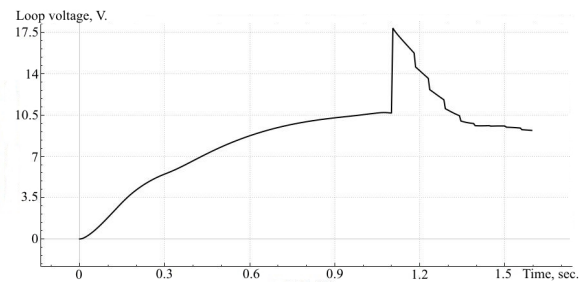
Figure 5. The loop voltage in the center of the breakdown area
