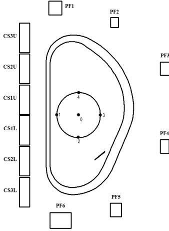
Figure 1. System poloidal coils and configuration of the passive structures in ITER. Point 0–4 are the characteristic points of the breakdown area.
