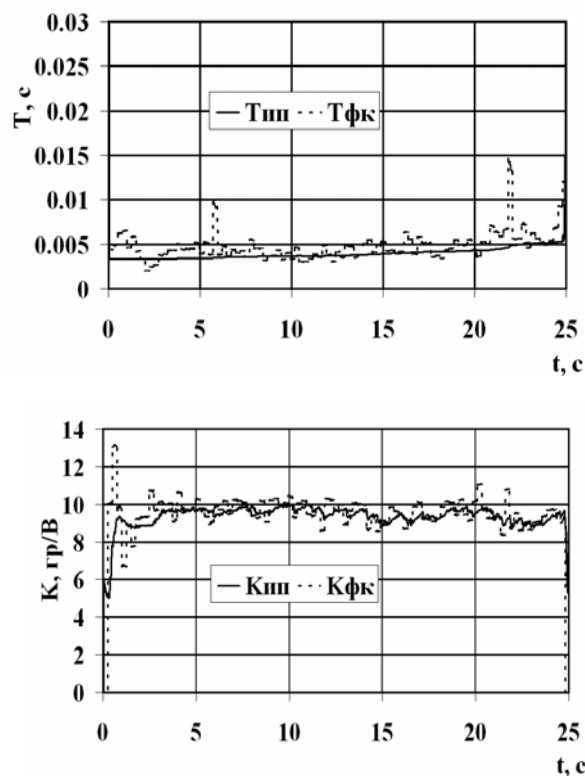
Fig. Results of estimation of time constant and servo transfer ratio by means of the invariant immersion method ( T_{ИП} , K_{ИП} ) and the Kalman filtration ( T_{ФК} , K_{ФК} )
